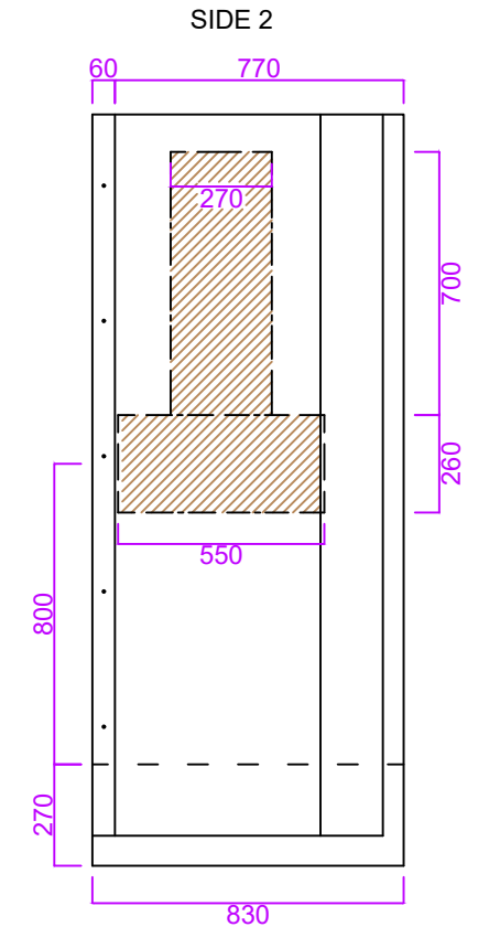
PLINTH DETAIL
